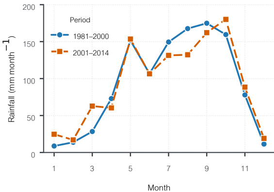
(a) Monthly climatology
