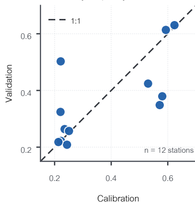
(c) Wet-day frequency
