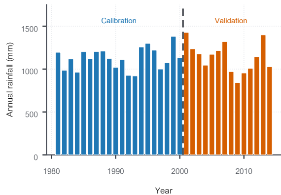
(b) Annual rainfall
